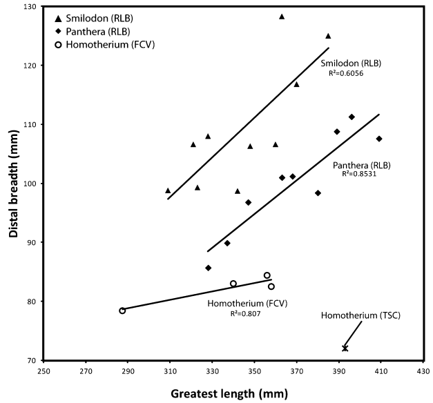
Fig. 8. Measurements on humeri from P. atrox , Smilodon and H. serum . RLB = Rancho la Brea (Merriam & Stock 1932); FCV = Friesenhahn Cave (Rawn-Schatzinger 1992); TSC = Tyson Spring Cave.
