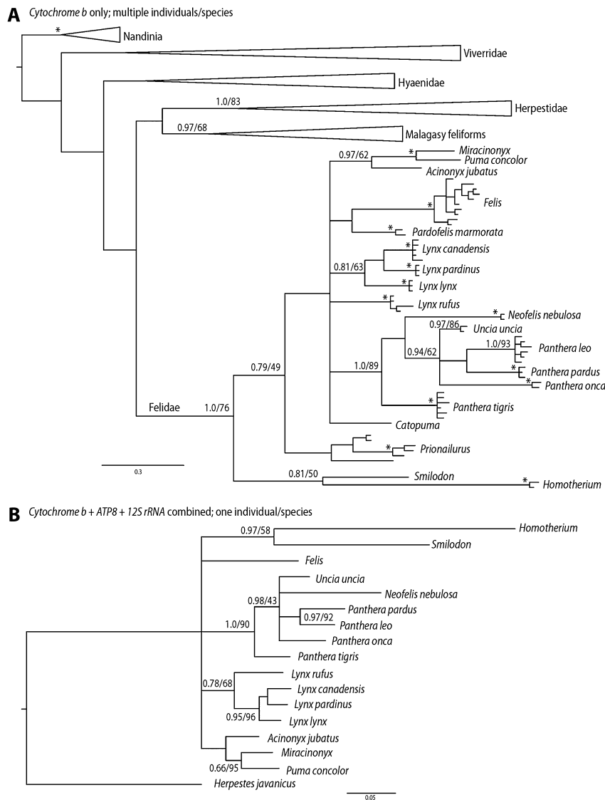
Fig. 9. Molecular phylogenetic placement of Homotherium within Feliformia. Bayesian phylogeny of (A) extant feliforms plus Homotherium , Smilodon and Miracinonyx based on cytochrome b data, including multiple individuals per species; clades outside Felidae are collapsed, or (B) three genes combined, sampling only one individual per species. The sequences included in this analysis are found in Table S2. Support values on branches indicate Bayesian posterior clade probabilities/maximum likelihood bootstrap proportions. Stars represent nodes that were supported by BPP \geq 0.98 and MLBP \geq 95\% ; unnumbered clades received no support (BPP \leq 0.8 , MLBP \leq 60 ).
